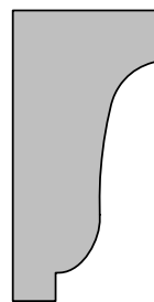
A&M # 1997 11/16" X 1-3/8"
