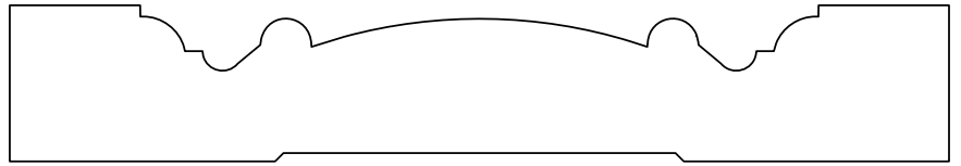
A&M # 2415 3/4" X 4-1/2"
