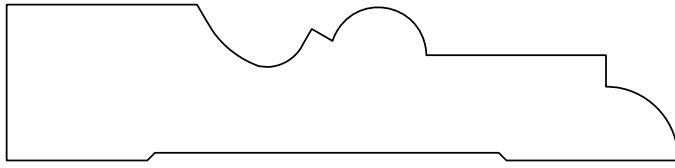
A&M # 3404 13/16" X 3-1/2"
