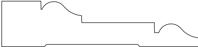
A&M # 30208 13/16" X 3-1/2"
