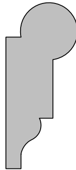
A&M # 8263 3/4" X 1-3/4"
