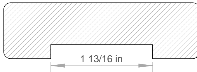
A&M # 6287 1" X 3-1/2"
