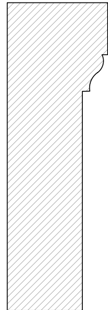
A&M # 4630 1-1/16" X 3-1/4"
