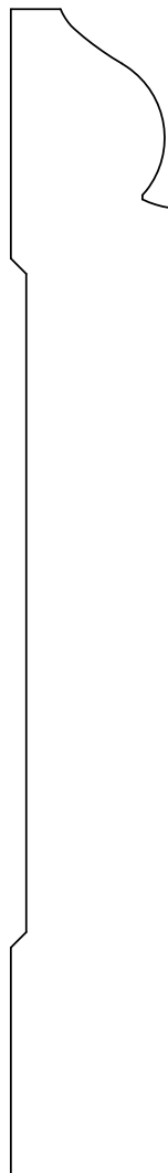
A&M # 1827 3/4" X 5-1/2"
