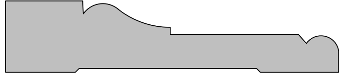
A&M # 3076 3/4" X 3-1/2"
