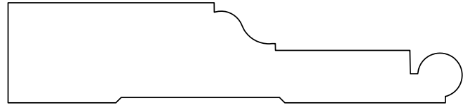
A&M # 3698 3/4" X 3-3/8"
