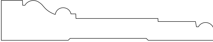
A&M # 3890 13/16" X 4-1/4"
