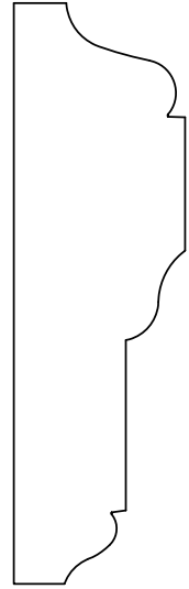
A&M # 4059 13/16" X 2-3/4"
