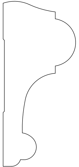
A&M # 4001 1-9/16" X 3-1/2"
