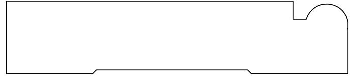
A&M # 3900 3/4" X 3-1/2"
